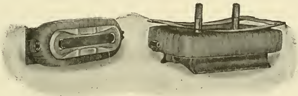
Fig. 34. Main Pole and Interpole Complete
